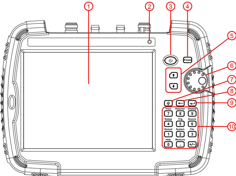
Figure 4-1 Front panel
